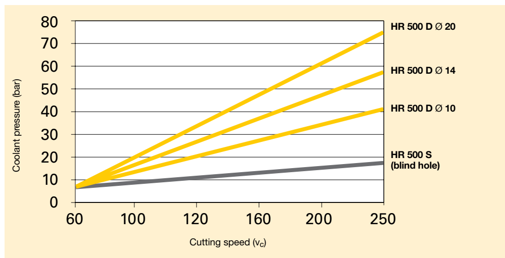
Coolant pressure - cutting speed valid for standard dimensions. Preconditions: sufficient capacity of coolant pump
